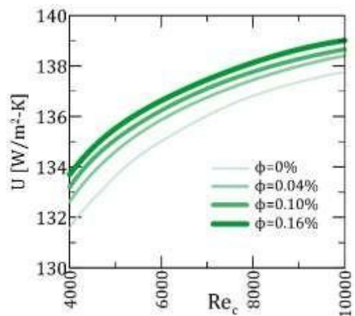
Figure 11. Overall heat transfer coefficient evaluated at different nanofluid concentrations for Re_a = 10000
