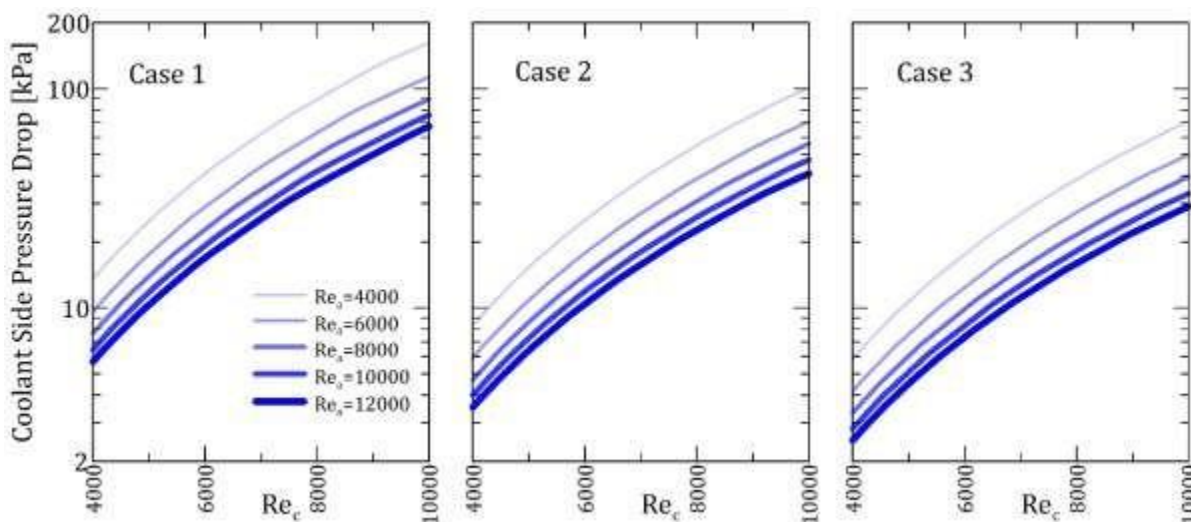
Figure 5. Effect of the compression ratio in each stage on the coolant-side pressure drop for different air Reynolds numbers
