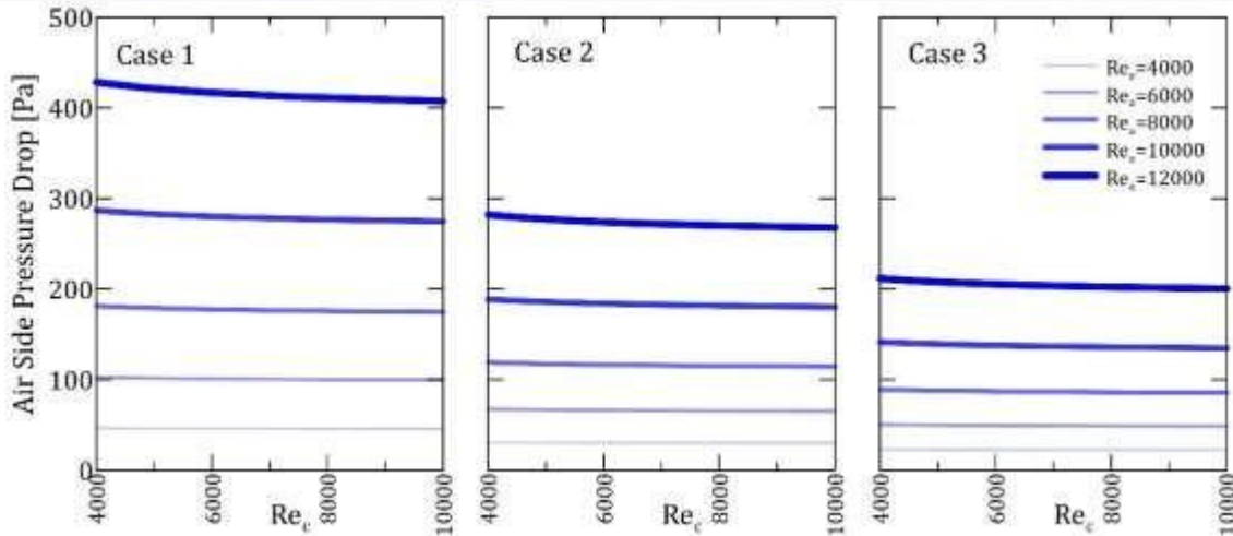
Figure 6. Effect of the compression ratio in each stage on the airside pressure drop for different air Reynolds numbers
