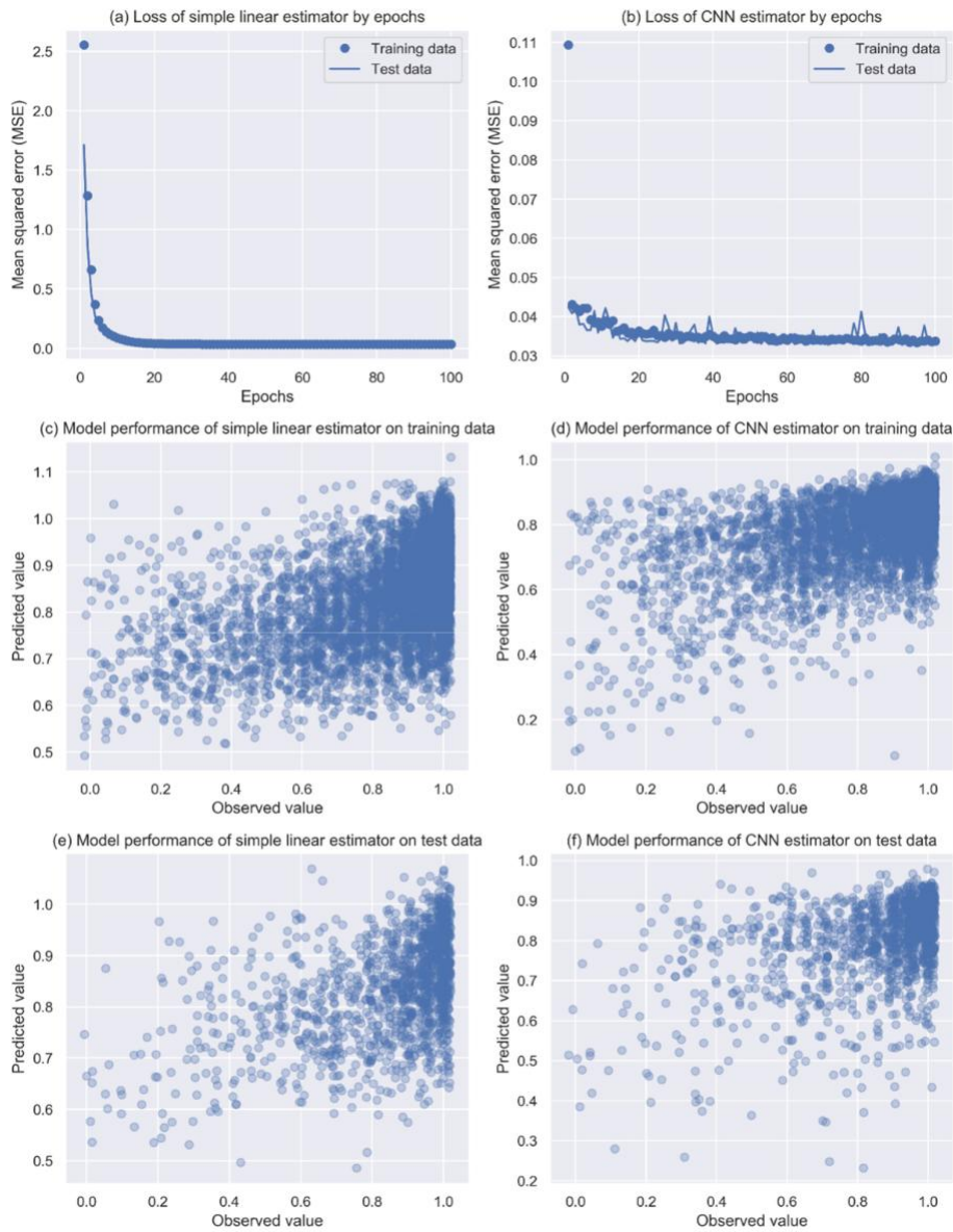
Figure 3. Model performance of the simple linear estimator and the CNN estimator. The dots in
