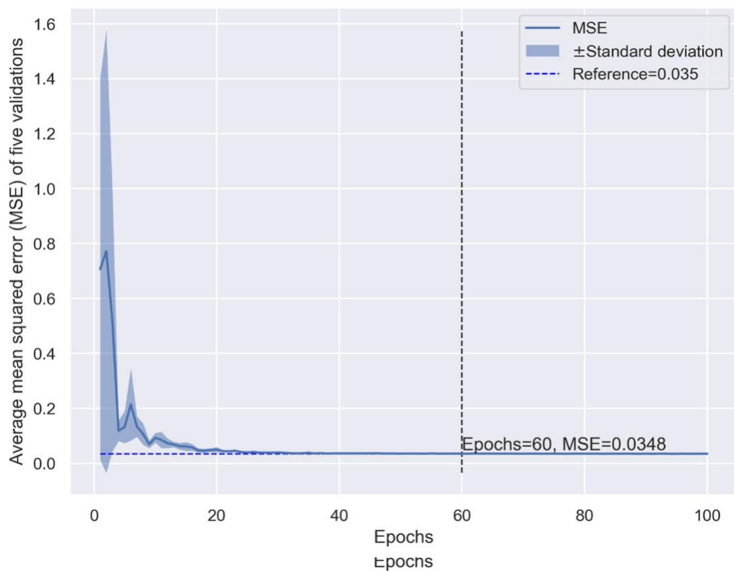
Figure 1. Performance of the convolution neural network (CNN) model in K-fold cross-validation. Figure 1. Performance of the convolution neural network (CNN) model in K-fold cross-validation. Figure 1. Performance of the convolution neural network (CNN) model in K-fold cross-validation.
